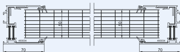
frame profile 455012 with front plate 492042/43
