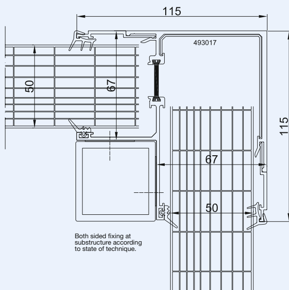
Corner profile 445072
