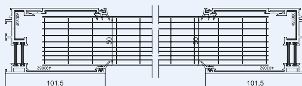
frame profile 455002 with front plate 492093
