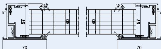
frame profile 454012 with front plate 492042/43
