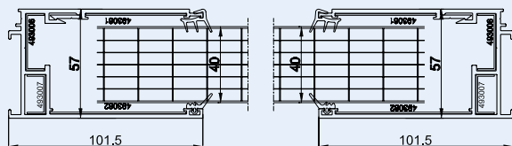
frame profile 454002 with front plate 492093
