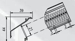
Lamela 30Z P1
