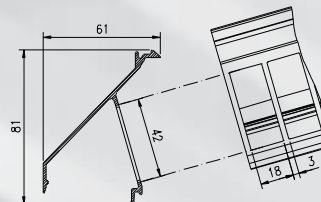
Lamela 50Z P2
