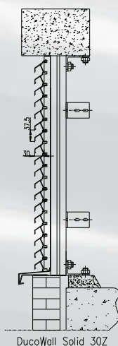
DucoWall Solid 30Z
