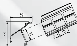
Lamela 30Z P2
